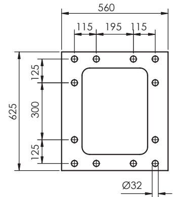
Gatenpatroon/hole pattern/ Bohrbild/motif de trous
